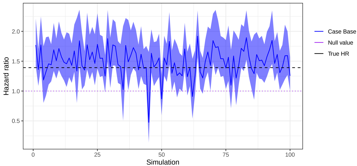
Case Base HR Confidence Intervals – Coverage: 0.864
